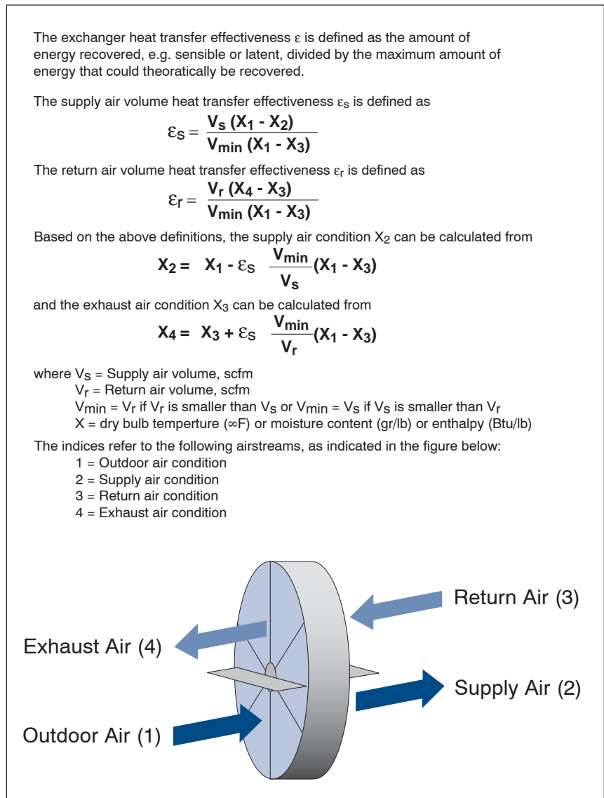
Figure 5. Definition of exchanger heat transfer effectiveness.
