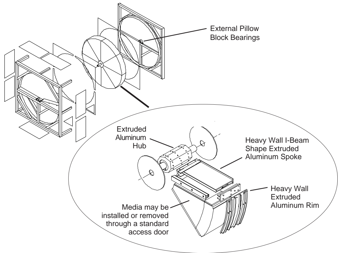
Hub & Spoke Construction Detail
