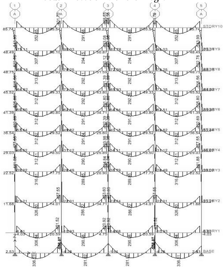
West Elevation Moment Diagram
