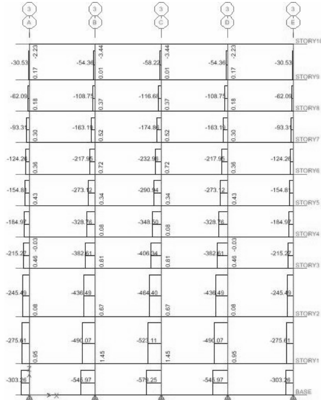
North Elevation Axial Loads
