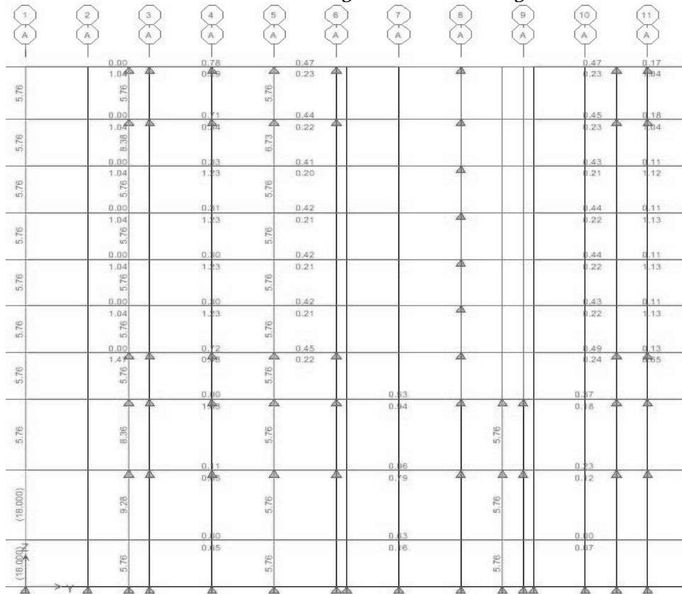
West Elevation Longitudinal Reinforcing
