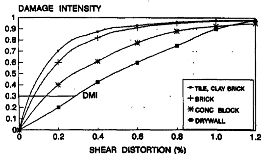
Fig. 4. Drift damage threshold—partitions.
