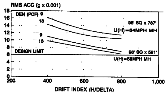
Fig. 5. RMS acceleration vs drift index.
