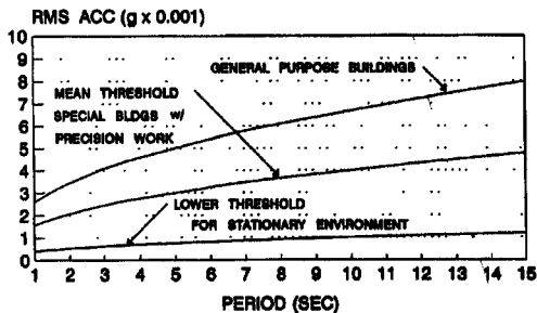
Fig. 10. RMS acceleration—ISO 6897-1984 5-yr return period.
