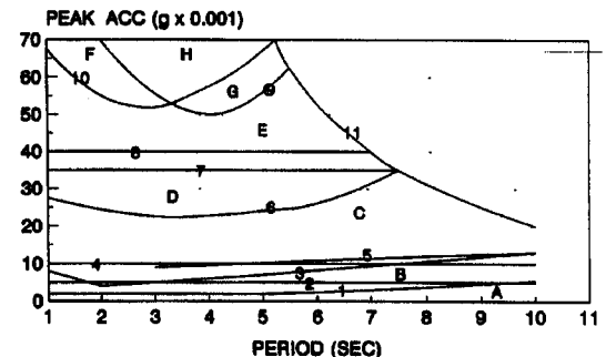
Fig. 8. Perception thresholds—peak acceleration.
