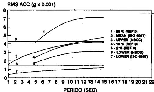
Fig. 7. Perception threshold—RMS acceleration.
