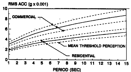
Fig. 11. Design standard—RMS acceleration 10-yr return period.
