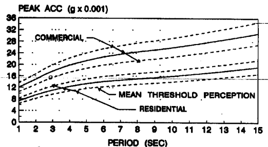
Fig. 12. Design standard—peak acceleration 10-yr return period.
