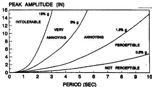
Fig. 6. Tolerance thresholds proposed by Chang.
