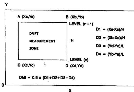
Fig. 1. Drift measurement index (DMI)
