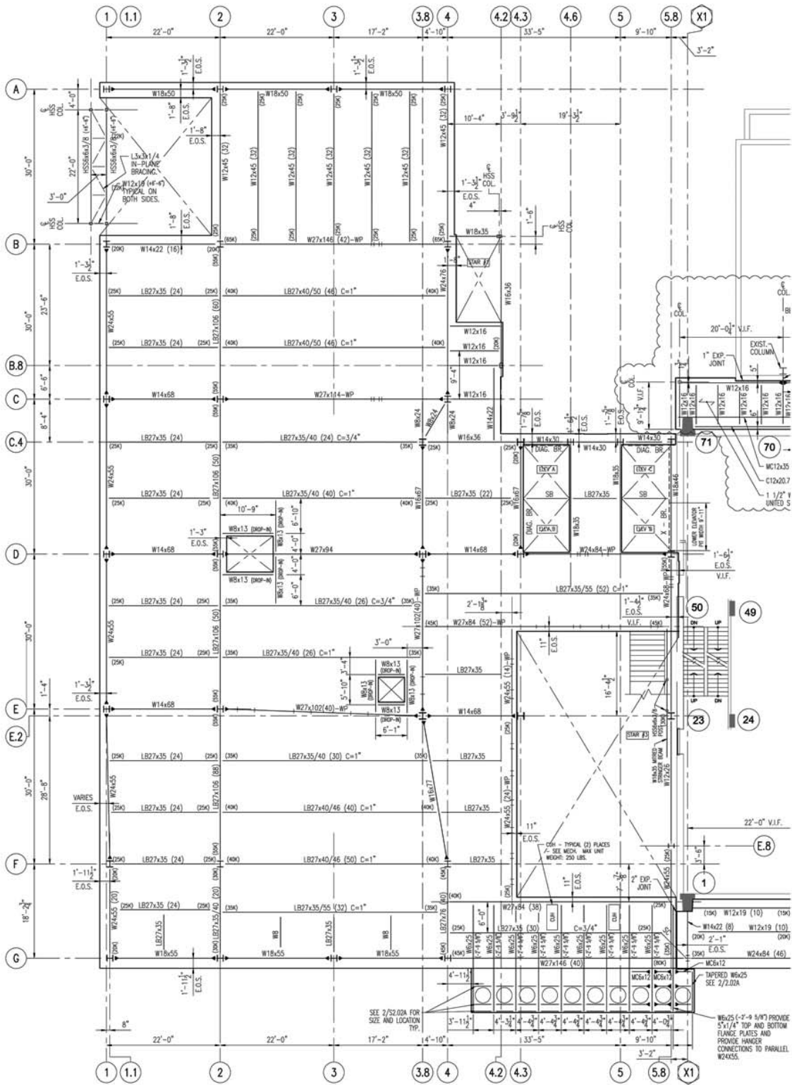
Typical Ambulatory Center Floor Framing Plan
