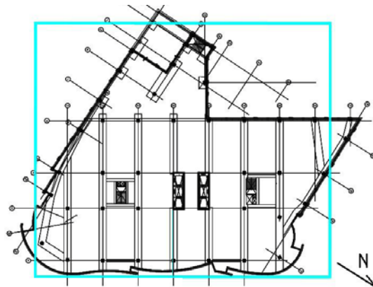
Figure 13: Initial Wind Load Determination
