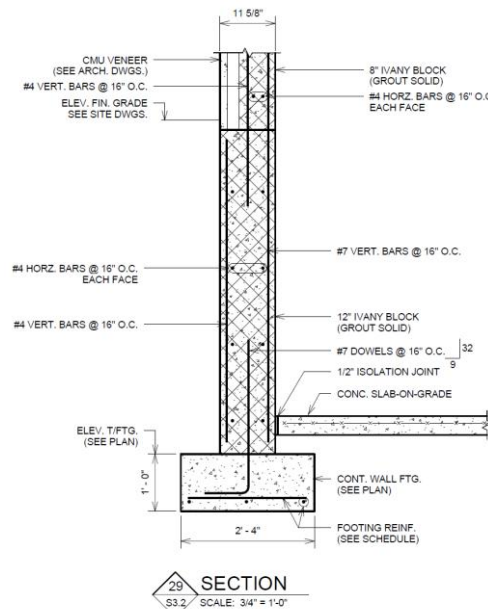
Figure 2: Typical Ivany Block Wall Courtesy of WTW Architects (Page S3.2)
