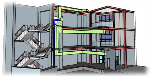
Figure 13: Sketch up Model of vertical chase in lobby
