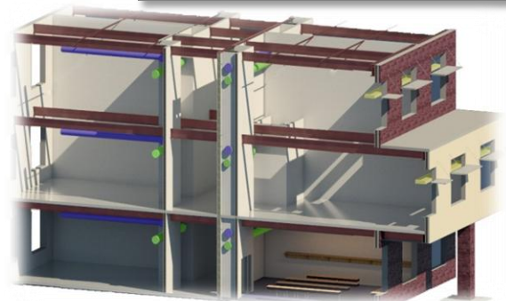
Figure 18: Ductwork running along hallway in the lateral chase.
