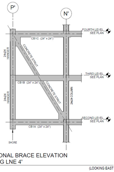
FIGURE 9: TYPICAL CONCRETE DIAGONAL BRACES
