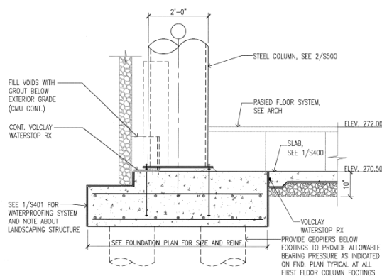
② STEEL COL. BRG. AT EXT. FOOTING ON GRID LINE C 3/8"=1'-0"
