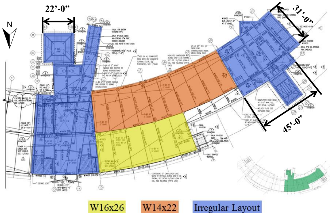
Figure 7 | Comparison of typical framing layout (yellow and orange) to irregular framing layout (blue), with a few general building dimensions (Drawing 1/S102a)
