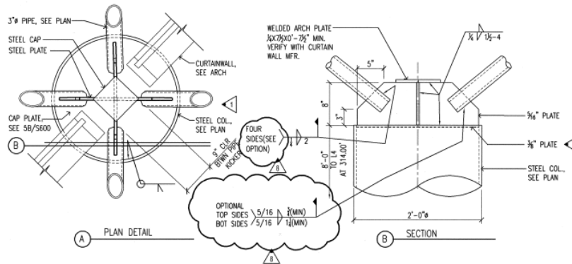
5 TYPICAL FLARE-OUT PIPE SUPPORT DETAIL 1/8" = 1'-0" 11"
