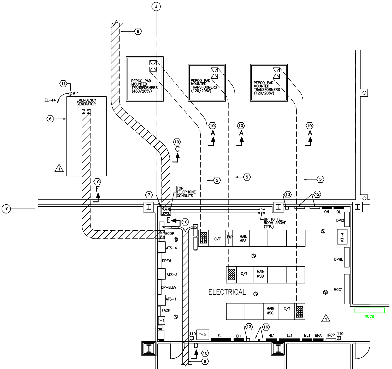
7 MAIN ELECTRICAL ROOM E3.01 SCALE: 1/4" = 1'-0" (LOWER LEVEL)
