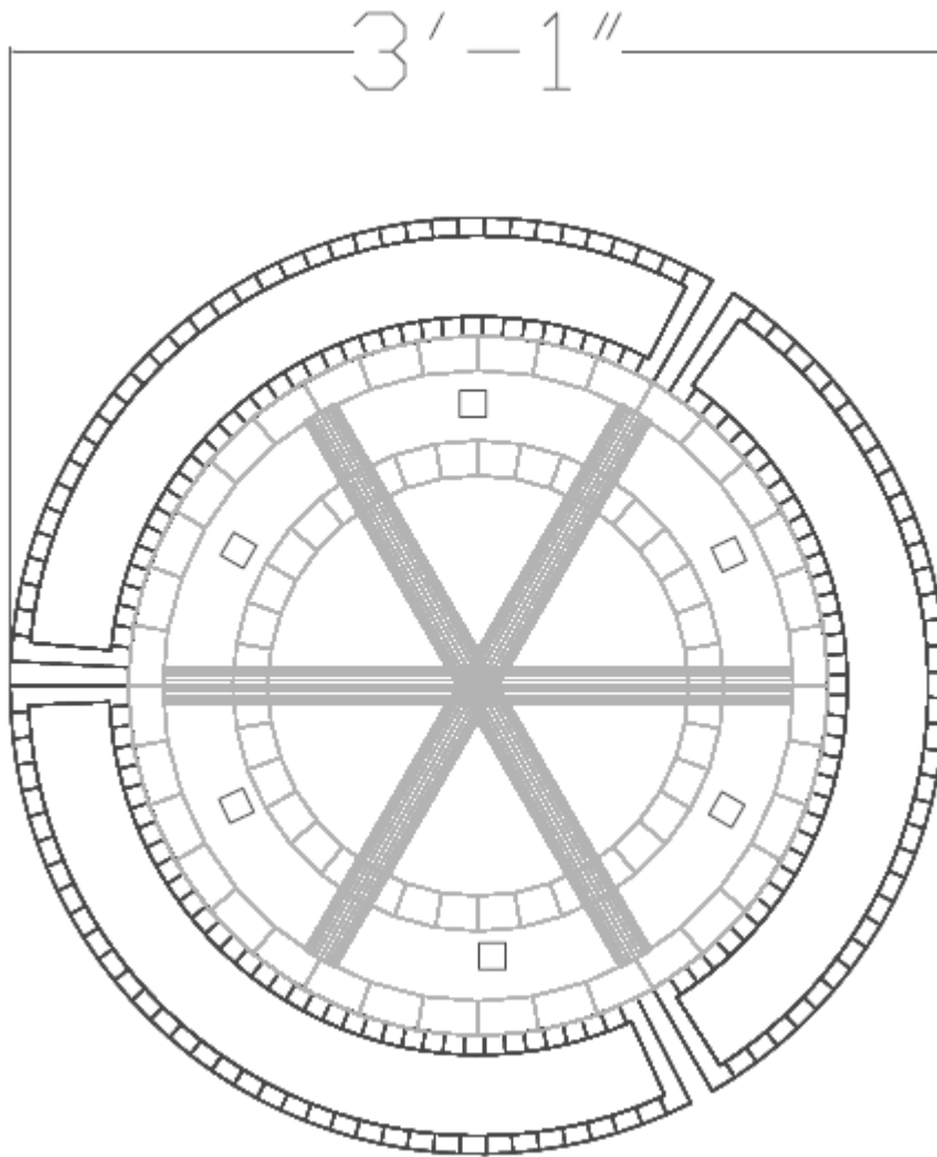
Top View Dimension
