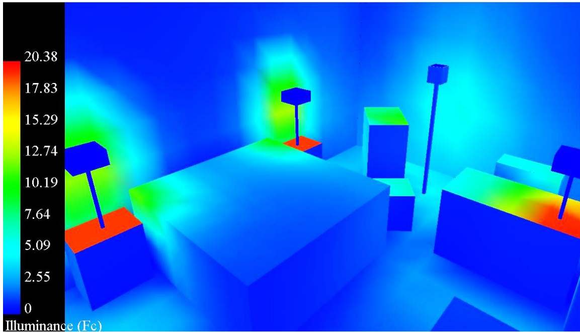
Figure H3 - Base Case Illuminance
