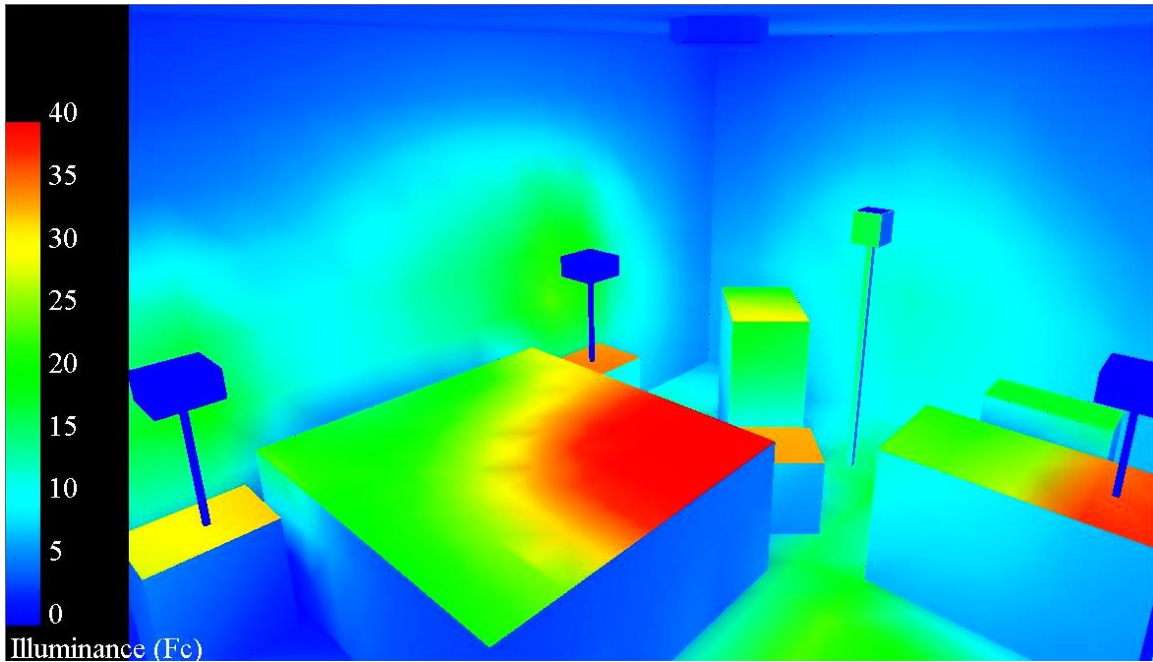
Figure H15 - Option 6 Illuminance
