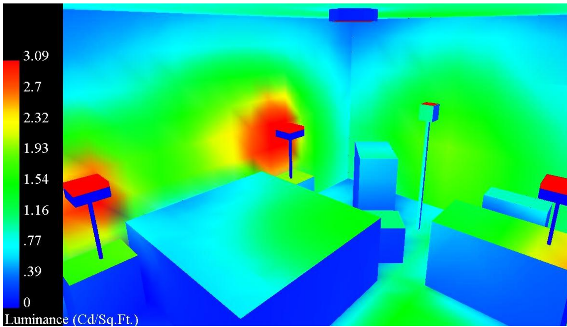
Figure H16 - Option 6 Luminance
