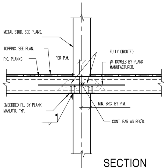
Figure 5-1 Hollow core plank ends spliced and resting on light gauge steel stud framed walls.
